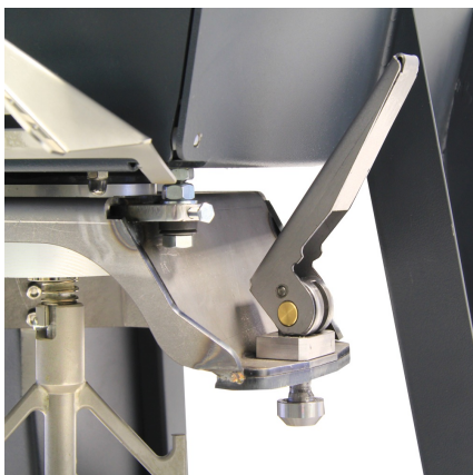
65-L0512 - Detail of the quick bowl mounting device
